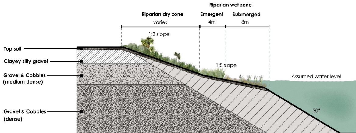
Figure 5: Showing slope margins to be created in order to rehabilitate the edges of the waterbody
